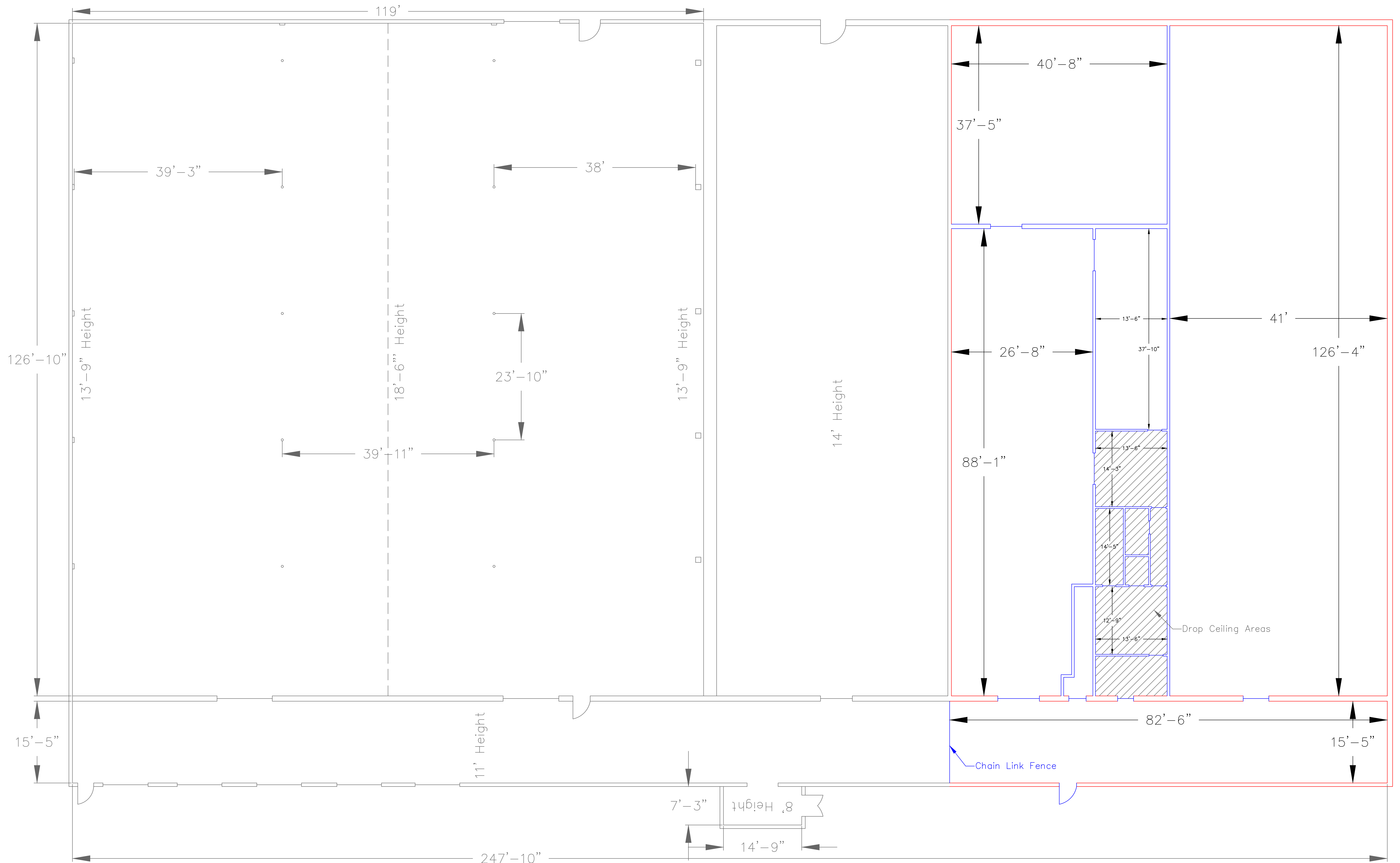
Rome Floyd County Recycle Center Additional Fire Suppression Areas Scale: 1/8"=1
